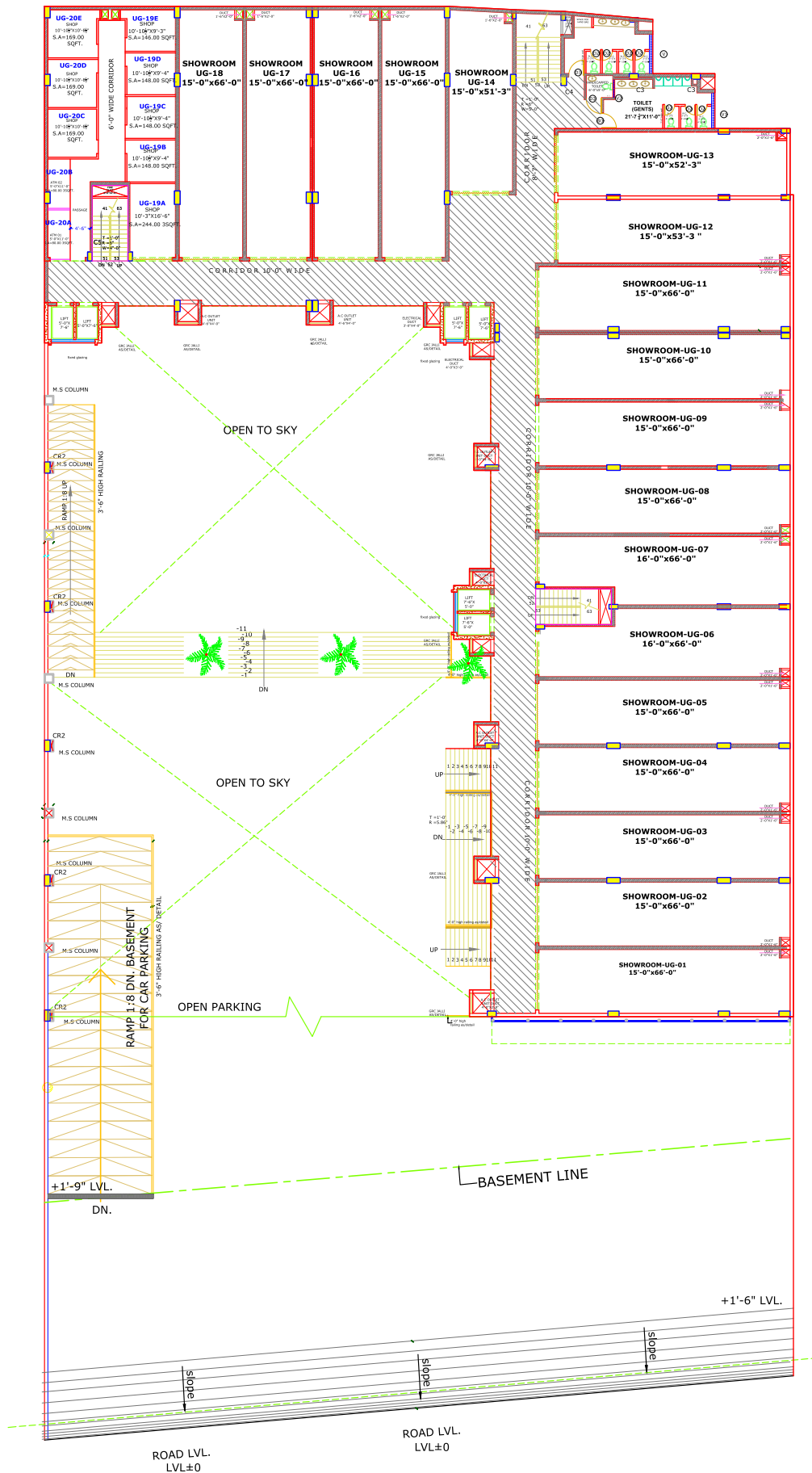
UPPER GROUND FLOOR PLAN
