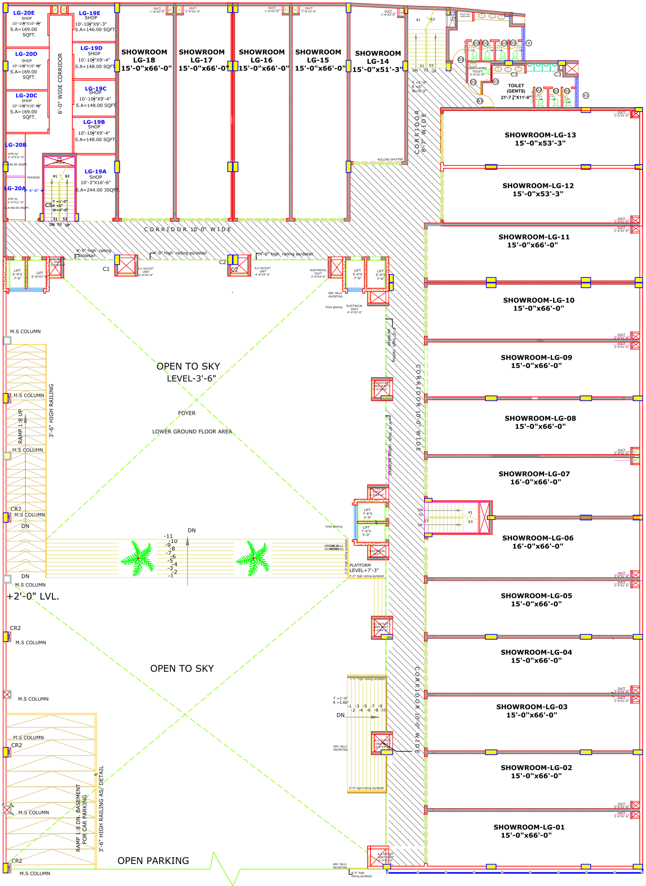
LOWER GROUND FLOOR PLAN
